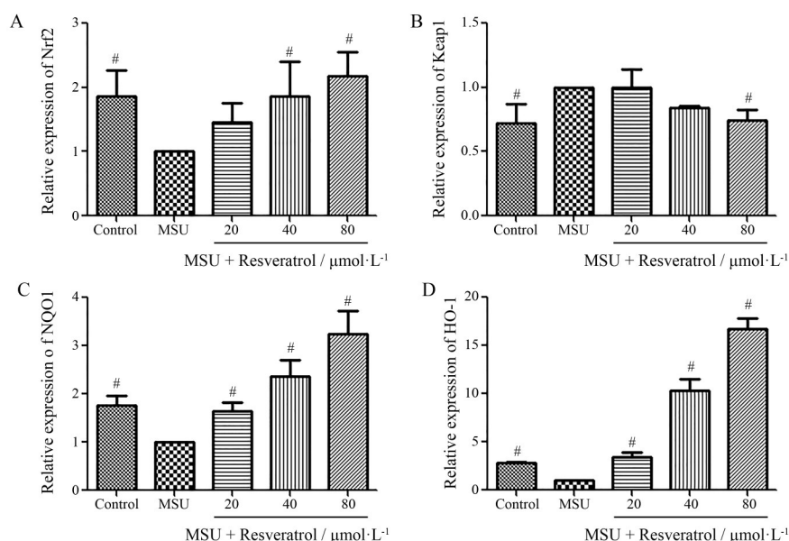
Figure 4 Effects of resveratrol on the expression of Nrf2, Keap1, NQO1, HO-1 mRNA stimulated by MSU in RAW264.7 cells. A, B, C, D: Relative expression of Nrf2, Keap1, NQO1, HO-1 mRNA were detected in RAW264.7 cells by Real time PCR, respectively. Nrf2: nuclear factor erythroid-2-related factor 2; Keap1: Kelch-like ECH-associated protein 1; NQO1: NAD(P)H quinoneoxidoreductase 1; HO-1: Heme oxygenase 1. n = 3 , \bar{x} \pm s . # P < 0.05 vs MSU group
